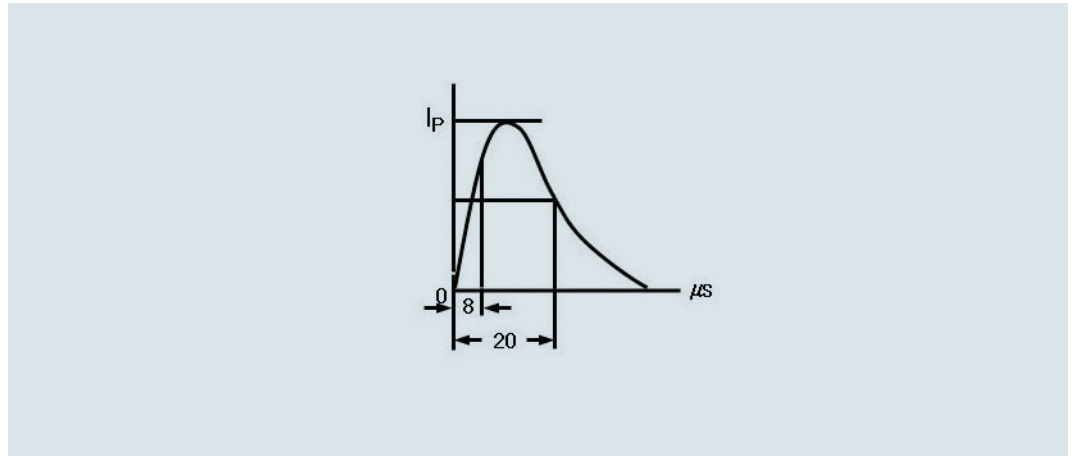
Surge current wave form
