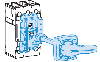
Door Mounted rotary operating handle [EHU, V, X-0, 2, 3, 5]
