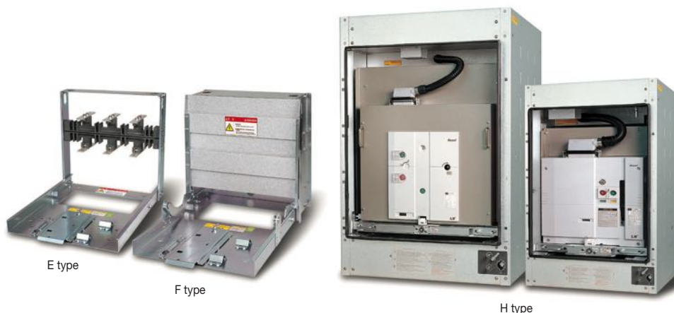
VCB Cradle type
