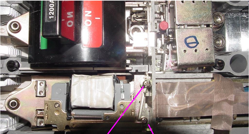
Screw(M4X35)
