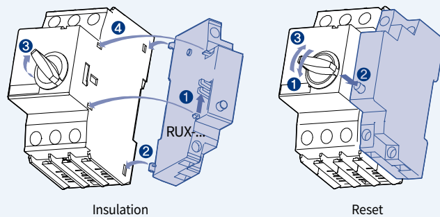
Insulation barrier
