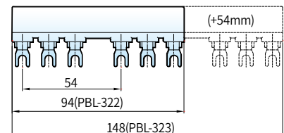
MMS-32H/32HI+PBL-32 PBL-322 (2 Terminals), PBL-323 (3 Terminals)
