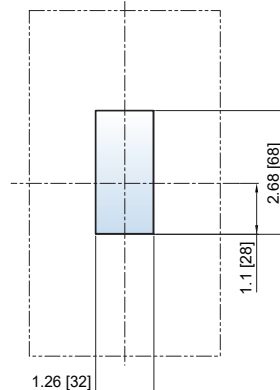
Cutouts A
