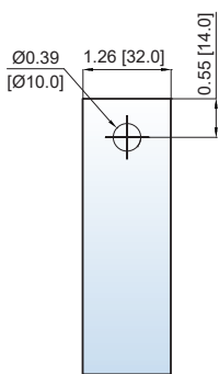
Conductor
