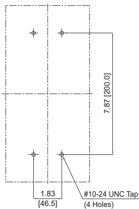
Panel drilling
