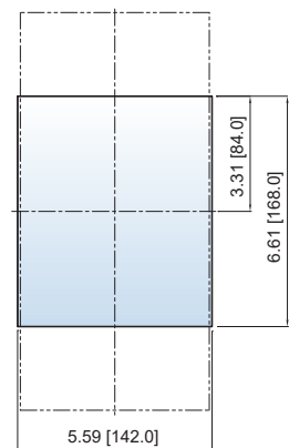
Cutouts B
