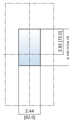
Cutouts A
