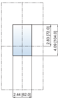
Cutouts A
