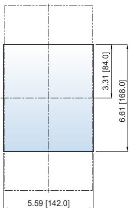
Cutouts B
